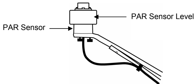
Figure 3: Leveling the PAR Smart Sensor on the Light Sensor Bracket
