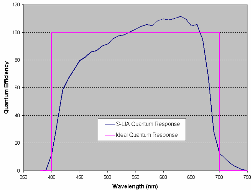
Figure 1: PAR Smart Sensor Typical Quantum Response
