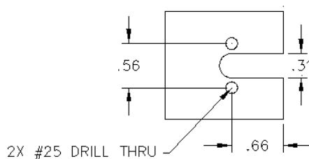
Figure 4: Recommended Mounting Plate Dimensions
